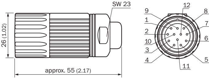
Dimensions in mm (inch)
