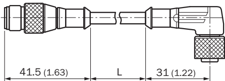
Dimensions in mm (inch)
