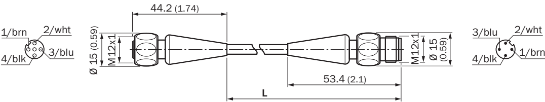
Dimensions in mm (inch)
