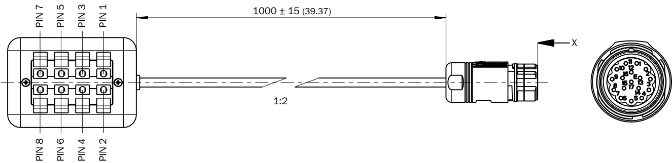
Dimensions in mm (inch)
