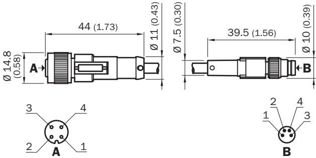
Dimensions in mm (inch)
