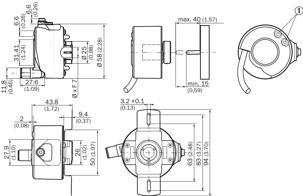
Dimensions in mm (inch) ① Status indicators
