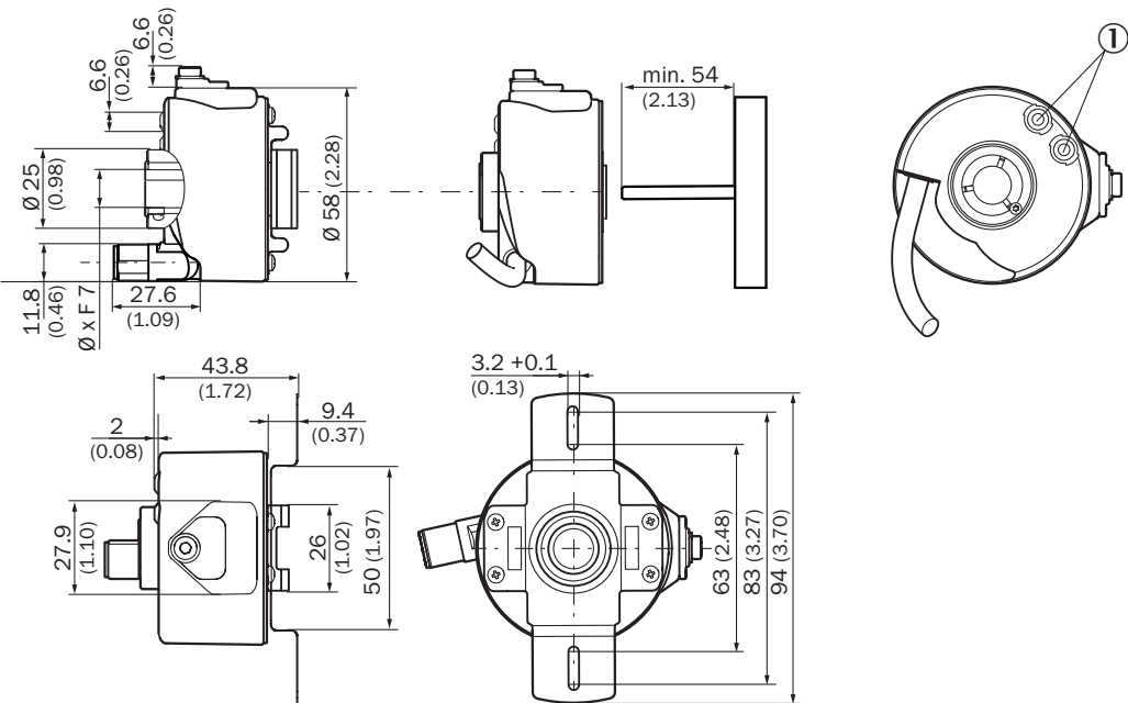
Dimensional drawing Through hollow shaft with rear clamping
