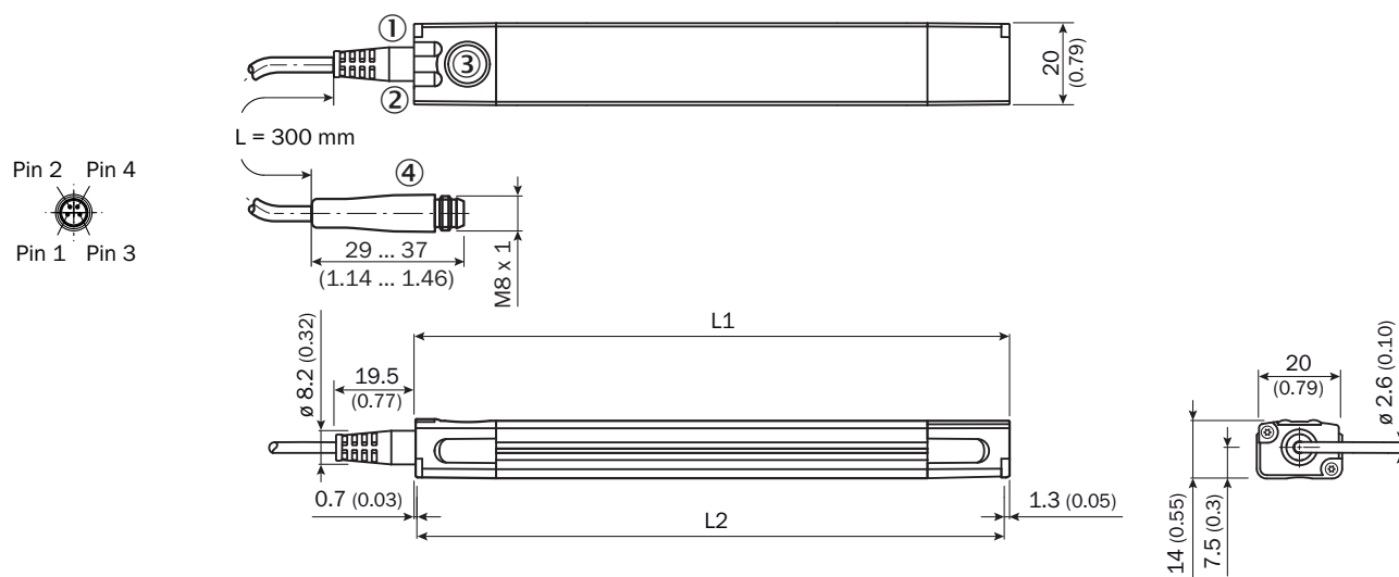
Dimensional drawing Cable with M8 male connector, 4-pin
