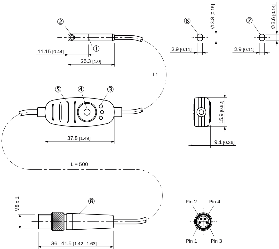
Dimensional drawing Cable with connector M8, with knurled nut
