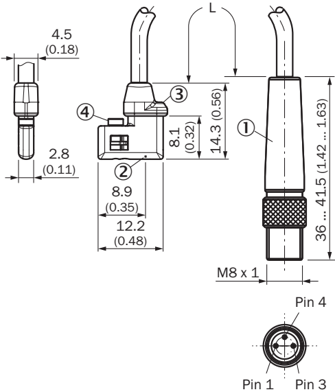
Dimensional drawing Cable with connector M8, with knurled nut
