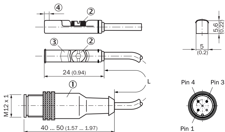
Dimensional drawing Cable with M12 male connector
