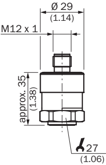
Dimensional drawing Housing with circular connector M12 x 1, IP67
