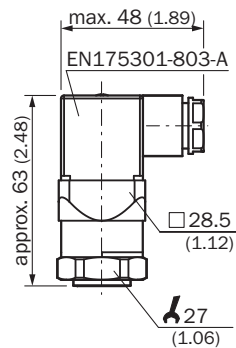
Dimensional drawing Housing with L-connector (DIN 175301-803 A), IP65
