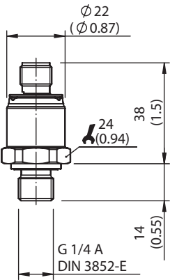
Dimensions in mm (inch)
