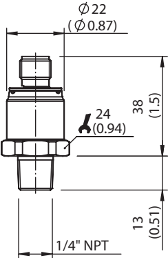
Dimensions in mm (inch)
