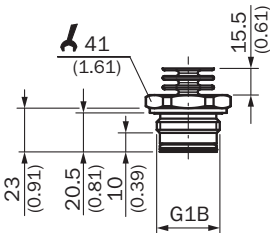
Dimensions in mm (inch)
