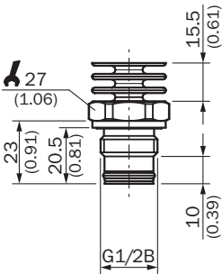
Dimensions in mm (inch)
