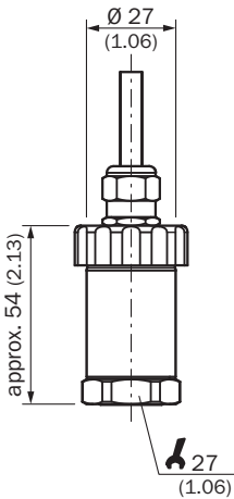
Dimensions in mm (inch)
