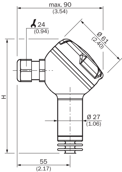
Dimensional drawing Stainless steel field case, compression fitting copper alloy, nickel plated, IP67
