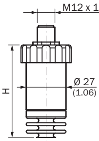
Dimensional drawing Housing with circular connector M12 x 1, IP67
