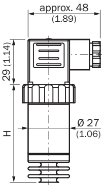
Dimensional drawing Housing with L-connector (DIN 175301-803 A), IP65
