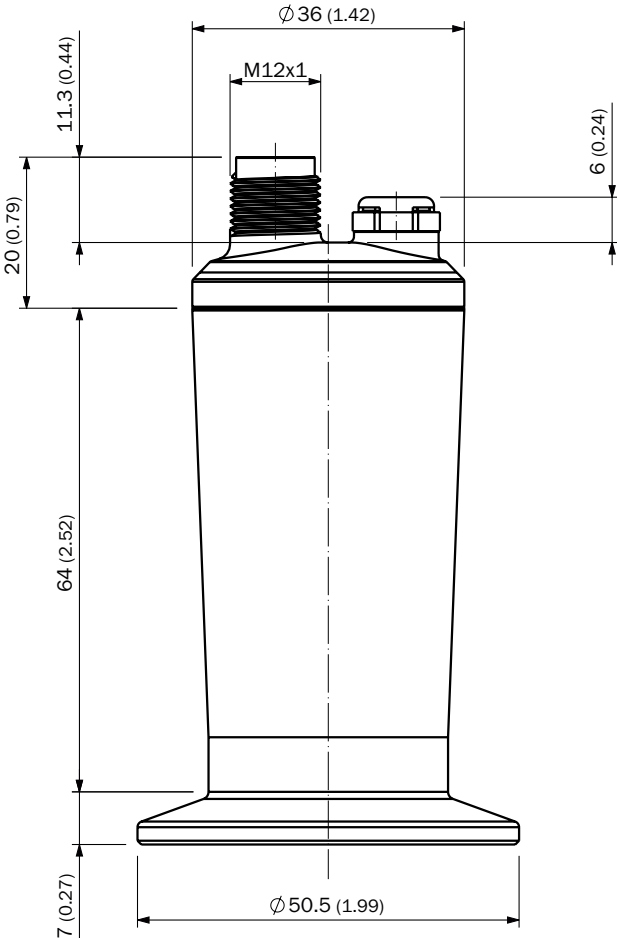
Dimensions in mm (inch)
