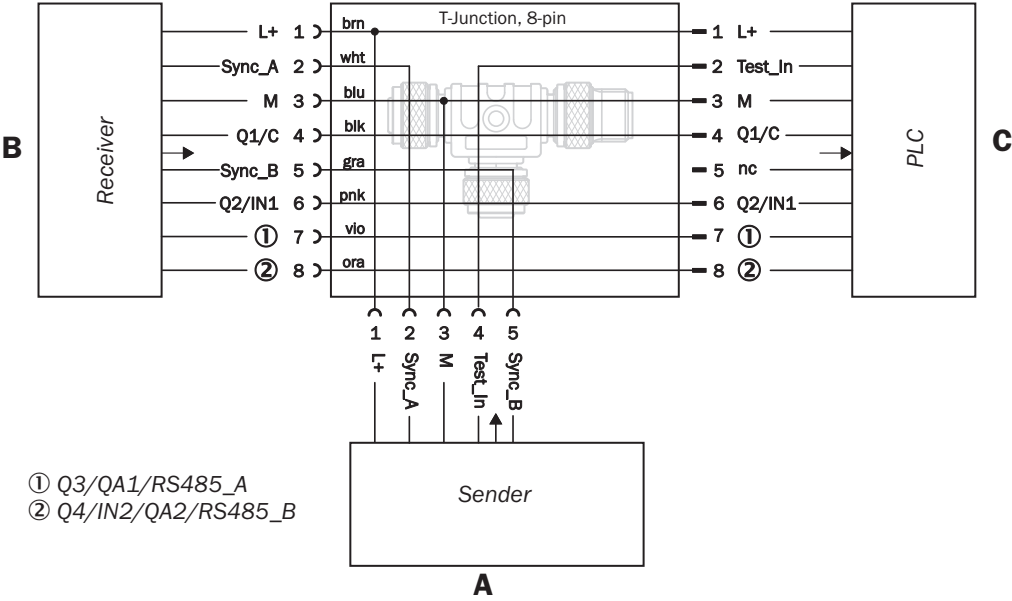
Connection diagram T-piece
