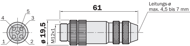
Dimensions in mm (inch)
