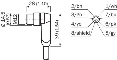
Dimensions in mm (inch)
