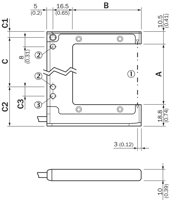
Dimensional drawing WFE-xxxxxx1xx
