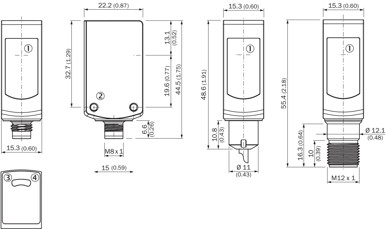
Dimensional drawing WL4S-3V, WLG4S-3V, without single teach-in button
