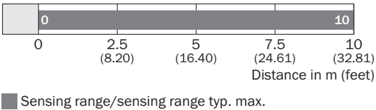
Sensing range diagram WS/WE12L-2, 10 m
