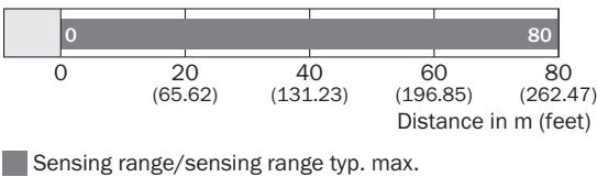
Sensing range diagram WS/WE12L-2, 80 m
