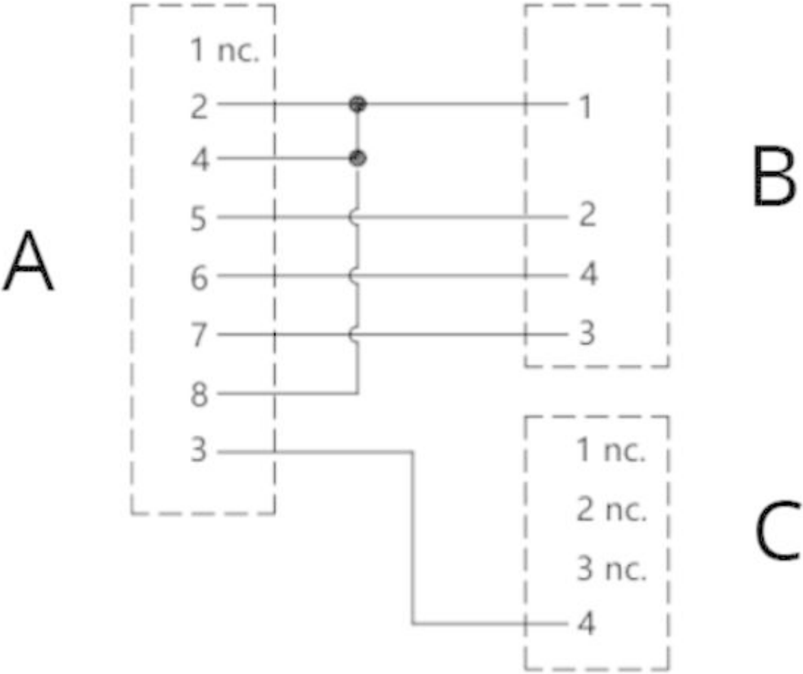
Connection diagram
