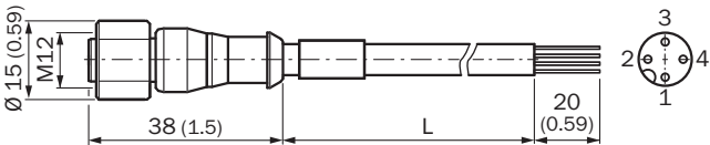
Dimensions in mm (inch) ① brn
