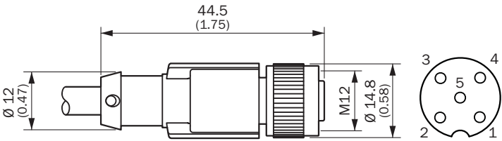
female connector M12 x1, straight, screened
