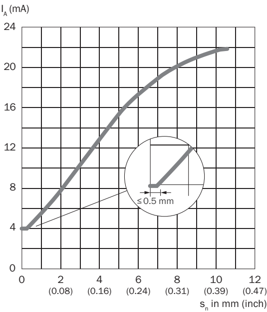
Response diagram Output current
