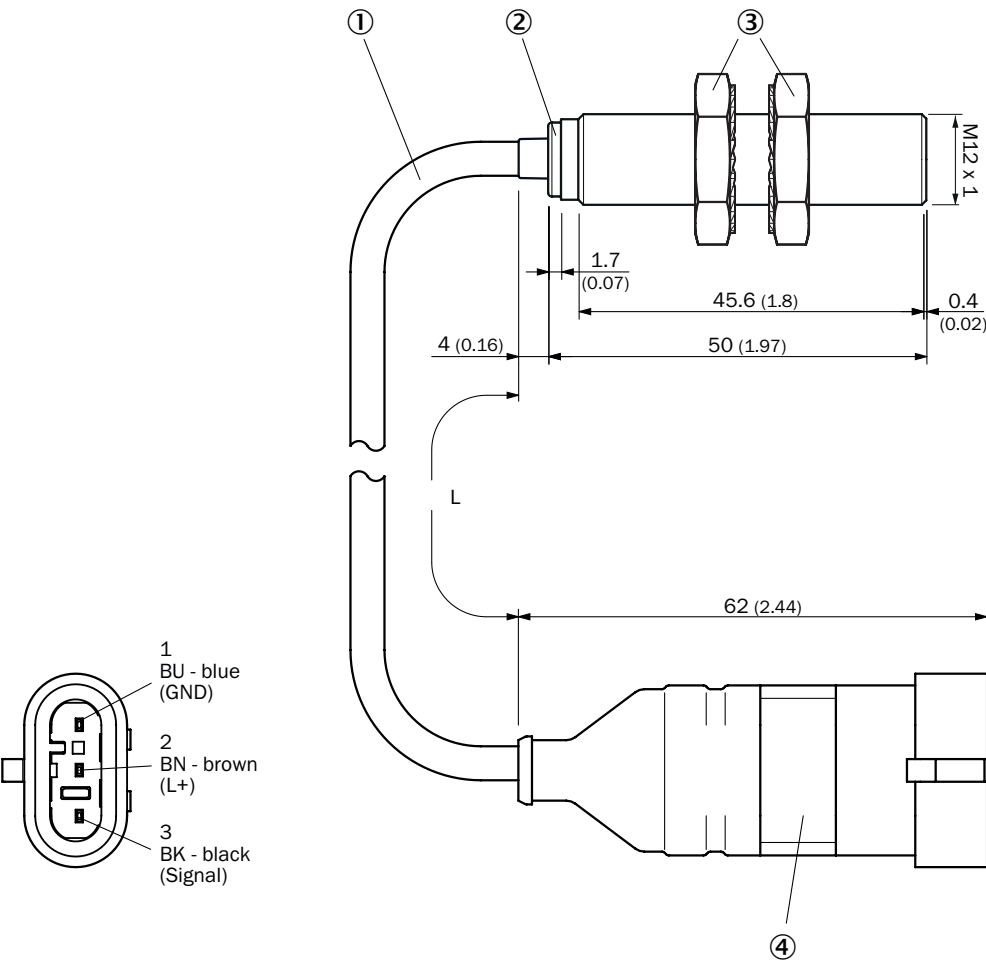
Dimensional drawing IMB12 standard variant, cable with AMP male connector, flush
