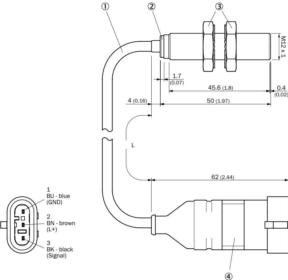
Dimensional drawing IMB12 standard variant, cable with AMP male connector, flush
