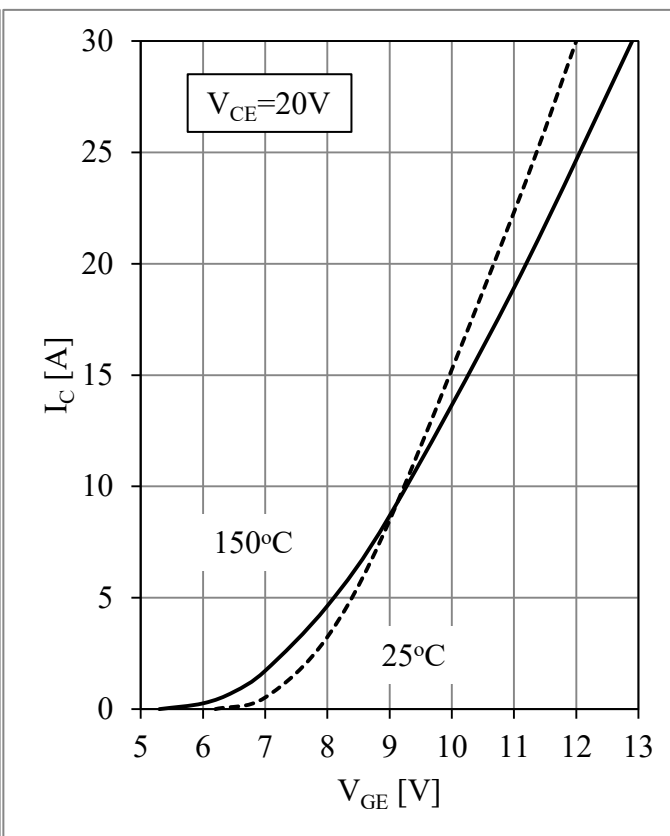
Fig 2. IGBT-inverter Transfer Characteristics
