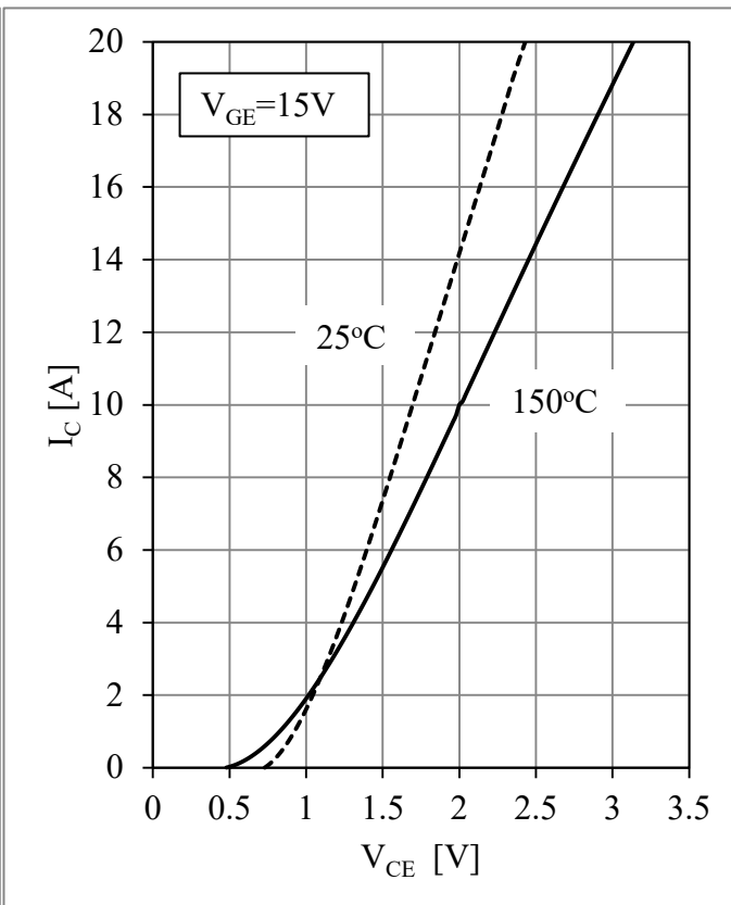
Fig 12. IGBT-brake Output Characteristics
