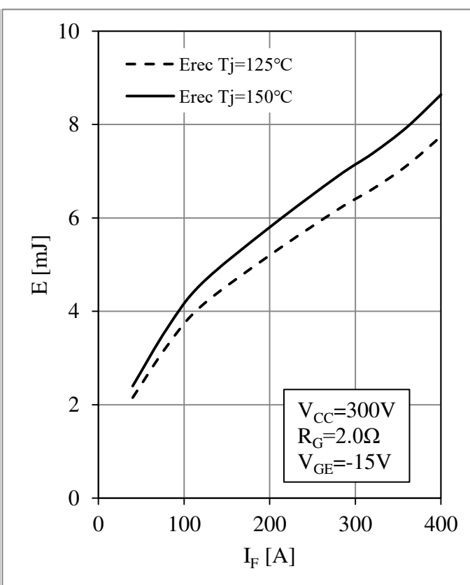
Fig 8. D1-D4 Diode Switching Loss vs. I_F
