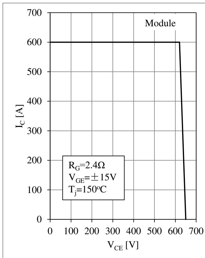
Fig 5. T2 T3 RBSOA
