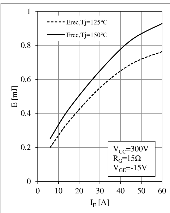
Fig 8. D2 D3 Diode Switching Loss vs. I_F
