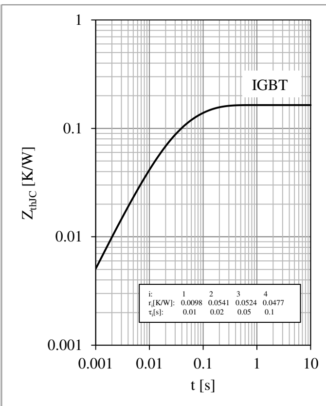
Fig 6. T2 T3 IGBT Transient Thermal Impedance
