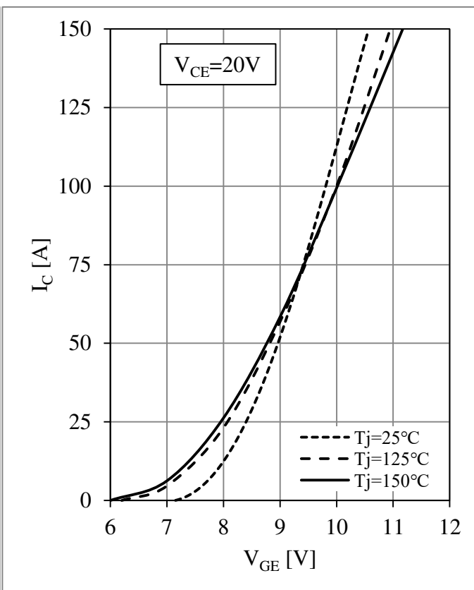
Fig 2. T1-T4 IGBT Transfer Characteristics
