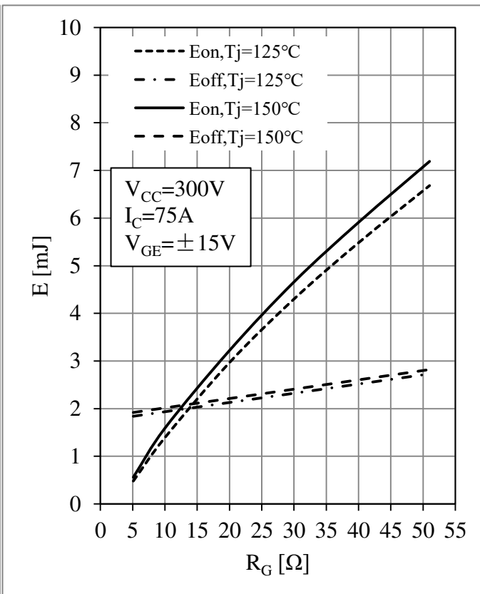
Fig 4. T1-T4 IGBT Switching Loss vs. R_G
