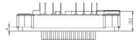
Dimensions in Millimeters
