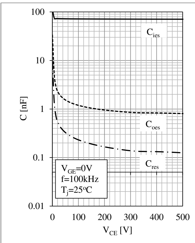
Fig 14. IGBT Capacity Characteristic
