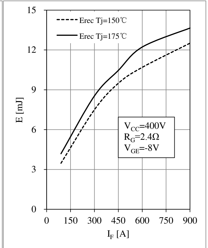
Fig 10. Diode Switching Loss vs. I_F
