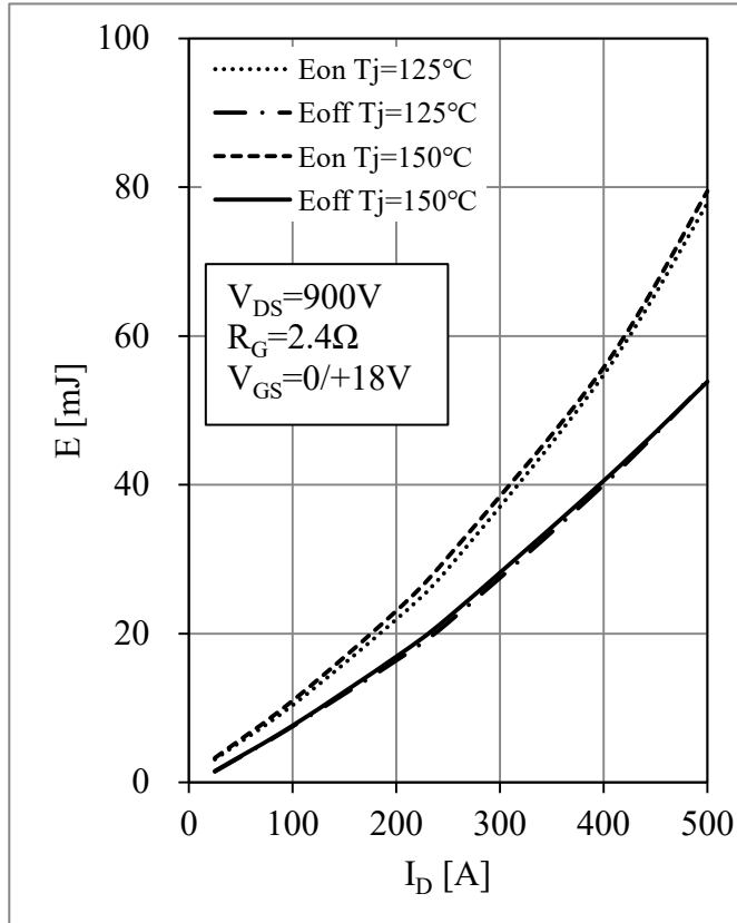
Fig 3. MOSFET Switching Loss vs. I_D
