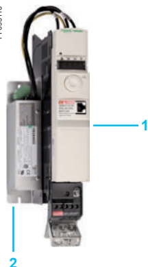
VW3A4422 + ATV32HU11N4
