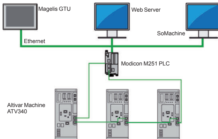
Integration in the SoMachine automation platform
