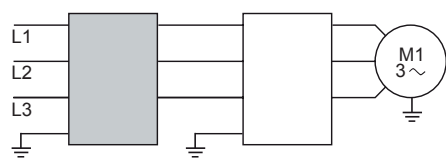
Additional EMC filter ATV340...N4 ATV340...N4E with integrated filter
