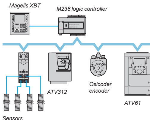
Example configuration on CANopen machine bus
