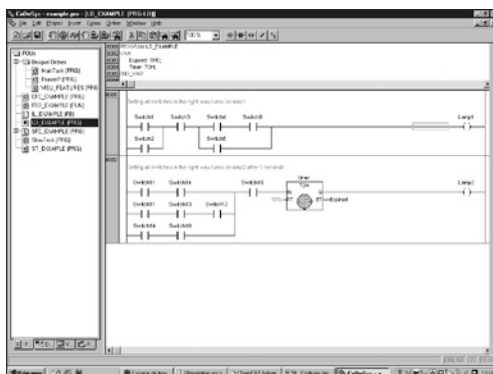
Ladder language programming example
