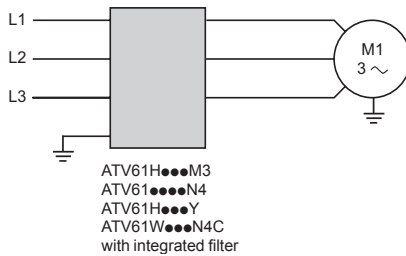
Altivar 61 drive with integrated EMC filter
