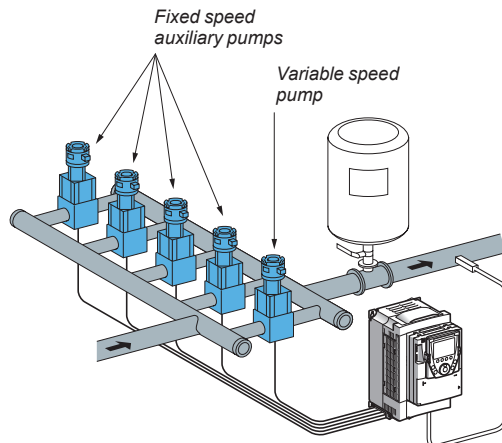
Example configuration of a pumping system with the VW3A3502 multi-pump card
