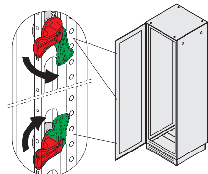
3-point locking with contradiirectional bolts
