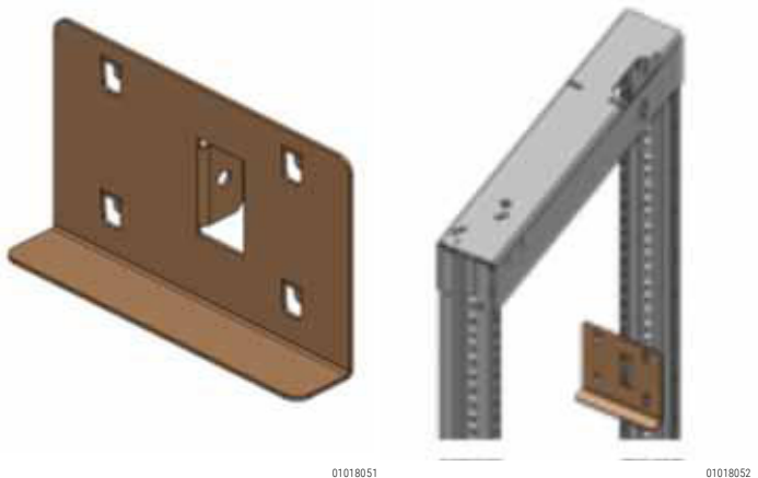
Sliding rails mounted on the swing frame
