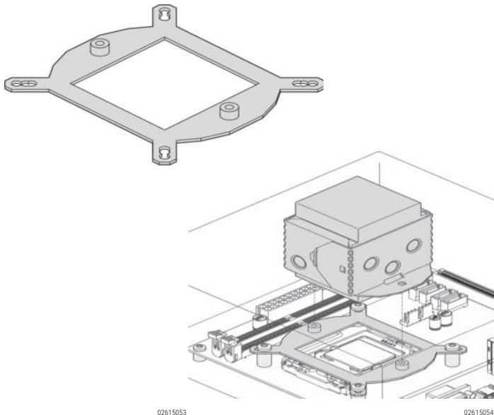
Bracket for Intel
