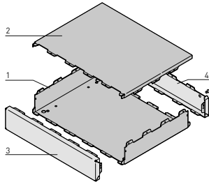
Plain case
