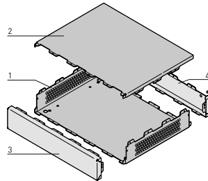
Perforated case
