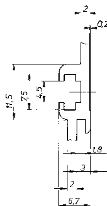
Detail "Y"
